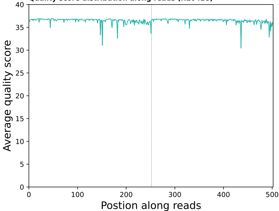
Quality score distribution along reads (R10428)
